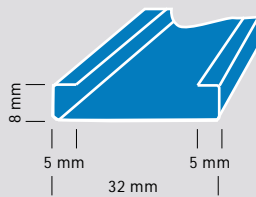
Furring Channel Code 91238
