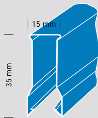
Top Cross Rail Code 91228
