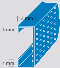
Super Furring Code 91149
